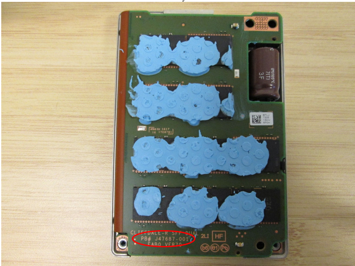
Secondary PCB:
